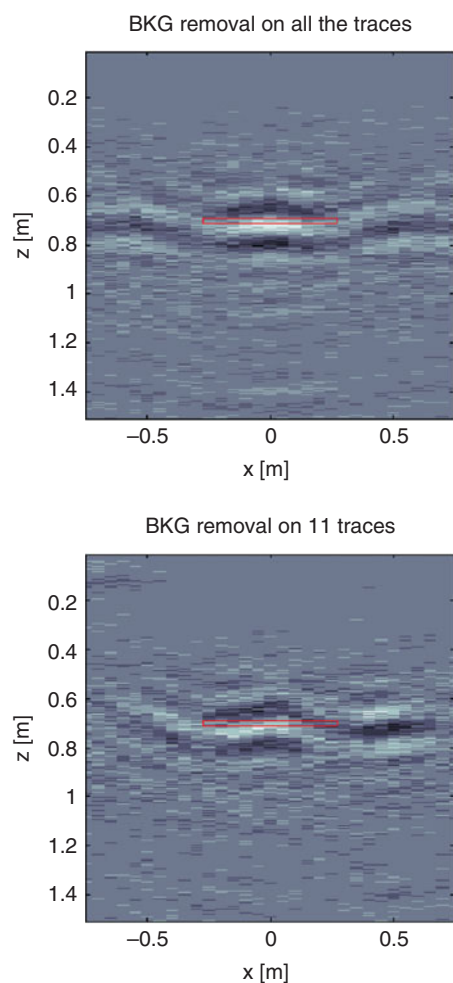
Figure 15.69. Upper panel: Migration performed with Reflexw after background removal on all the traces. Lower panel: Migration performed with Reflexw after background removal on 11 the traces. The scenario is that of Figure 15.65.
