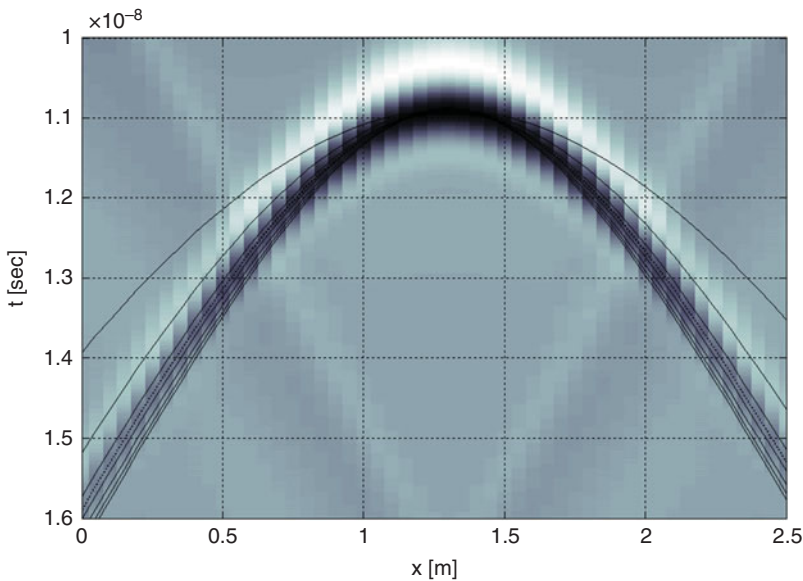
Figure 15.9. Diffraction curves considering the height of the observation line. Solid lines from top to bottom: Curves relative to trial relative permittivities ranging from 1 to 7. Dotted line: Heuristic best matching curve relative to the trial value 3.5.
