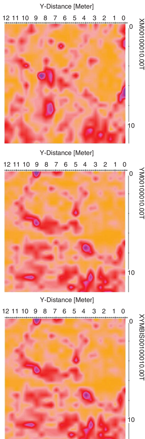
Figure 15.72. Depth slices at 47 cm obtained with Reflexw through a 2D migration-based processing. Upper panel: Result obtained from the B-scans parallel to only the x-axis. Middle panel: Result obtained from the B-scans parallel to only the y-axis. Lower panel: Result obtained from the B-scans parallel to both the x-axis and the y-axis. The axes are in meters. For color detail, please see color plate section.
