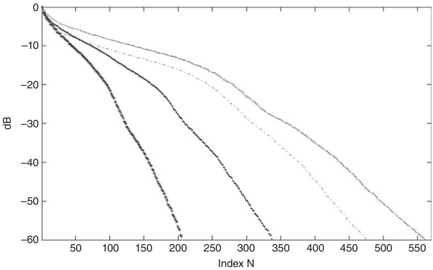
Figure 15.13. Singular values at variance of the spatial step: crosses (lower curve): s = 40 cm; dots: s = 20 cm; dots and dashes: s = 10 cm; solid line: s = 5 cm; dashes (almost indistinguishable from the solid line): s = 2.5 cm.
