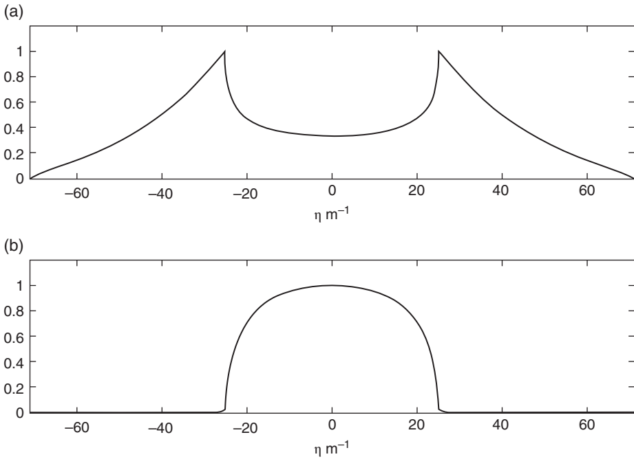
Figure 9.15. Comparison between the spectral weight at the soil and at height equal to the wavelength in air. In both panels, we have \epsilon_{sr}=4 , \mu_{sr}=2 , and f=600 MHz. Panel a: h=0 . Panel b: h=0.5 m. In the example at hand 2k_s=71.13 \text{ m}^{-1} and 2k_0=25.15 \text{ m}^{-1} .
