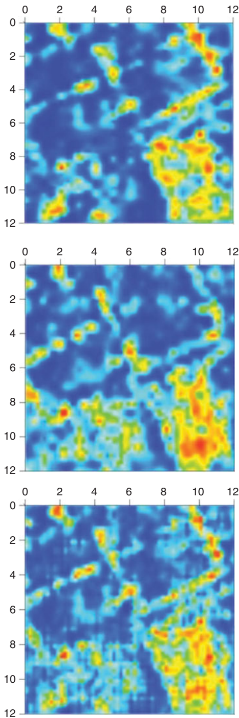
Figure 15.73. Depth slices at 47 cm obtained with GPRSLICE through 2D migration-based processing. Upper panel: Result obtained from the B-scans parallel to only the x -axis. Middle panel: Result obtained from the B-scans parallel to only the y -axis. Lower panel: Result obtained from the B-scans parallel to both the x -axis and the y -axis. The axes are in meters. For color detail, please see color plate section.
