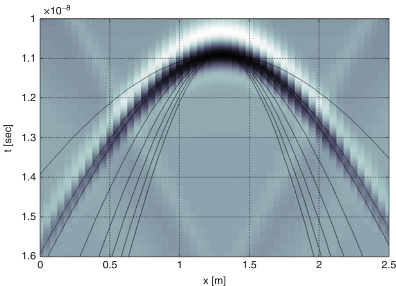
Figure 15.8. Diffraction curves neglecting the height of the observation line. Solid lines from top to bottom: Curves relative to trial relative permittivities ranging from 1 to 7. Dotted line: Heuristic best matching curve relative to the trial value 1.8.
