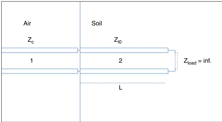
Figure 2.10. Circuitual scheme for a TDR probe.
