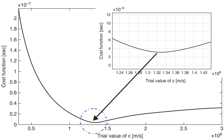
Figure 15.3. The cost function for a numerical evaluation of the propagation velocity.
